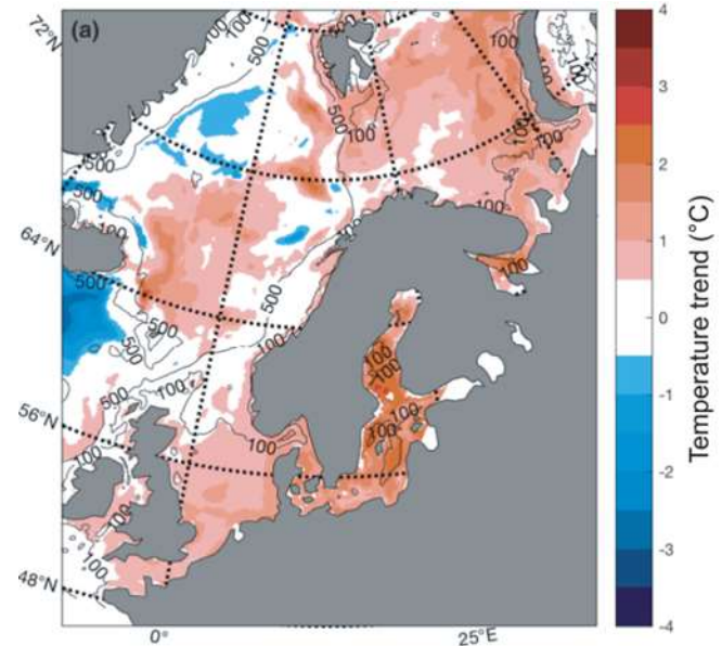
Projected change in sea surface temperature from 2010 to 2041 during wintertime (January–March) in the North East Atlantic.
